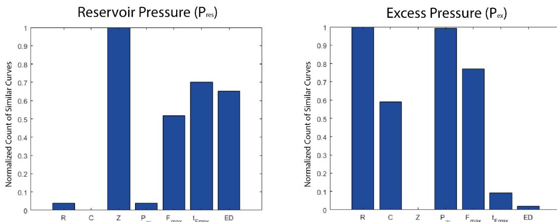
Figure 1: Results from sensitivity analysis: left P_{\text{res}} , right P_{\text{ex}} . The y-axis shows the normalized count of pairs of curves that remained similar (mean square error < 1 for P_{\text{res}} , mean square error < 0.25 for P_{\text{ex}} ), despite changes in the input parameter that are shown on the x-axis.
